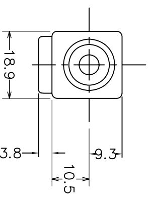
Insulator House Top View (for illustration)
