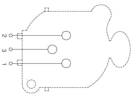
Schematic Layout
