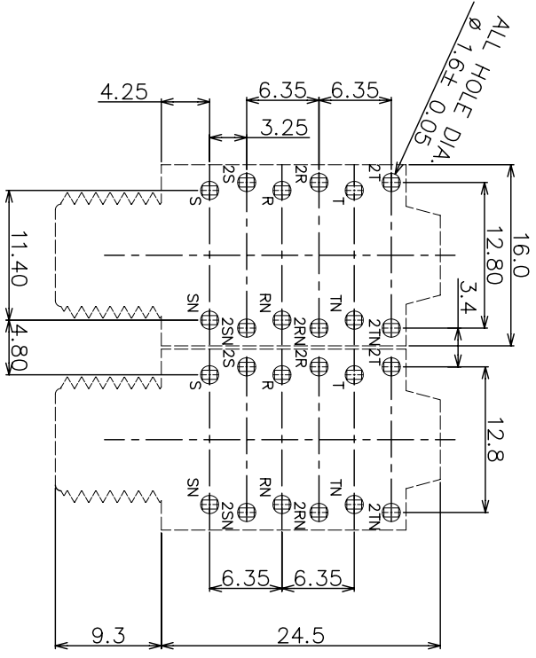
PCB LAYOUT
