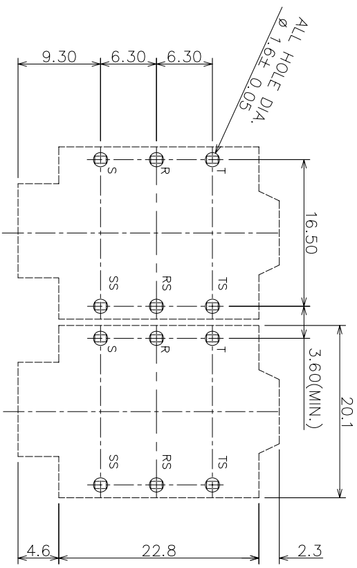
PCB LAYOUT
