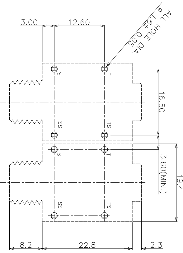
PCB LAYOUT
